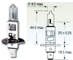
28. HALOGEN BULB 12V 60/55W PJ26.4T
