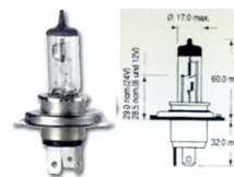
31. HALOGEN BULB 12V 60/55W P43T
