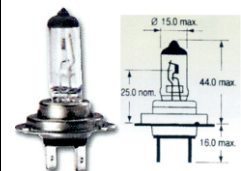
33. HALOGEN BULB 12V 55W PX26D
